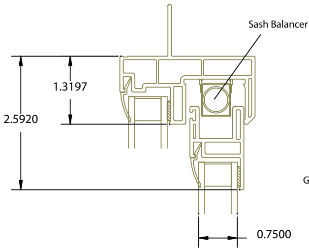
Horizontal Section
